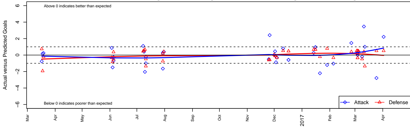
WA Rush G00 Dots are actual minus expected GF (blue circles) and GA (red triangles). Blue line is smoothed change in attack strength. Red is smoothed change in defense strength.
